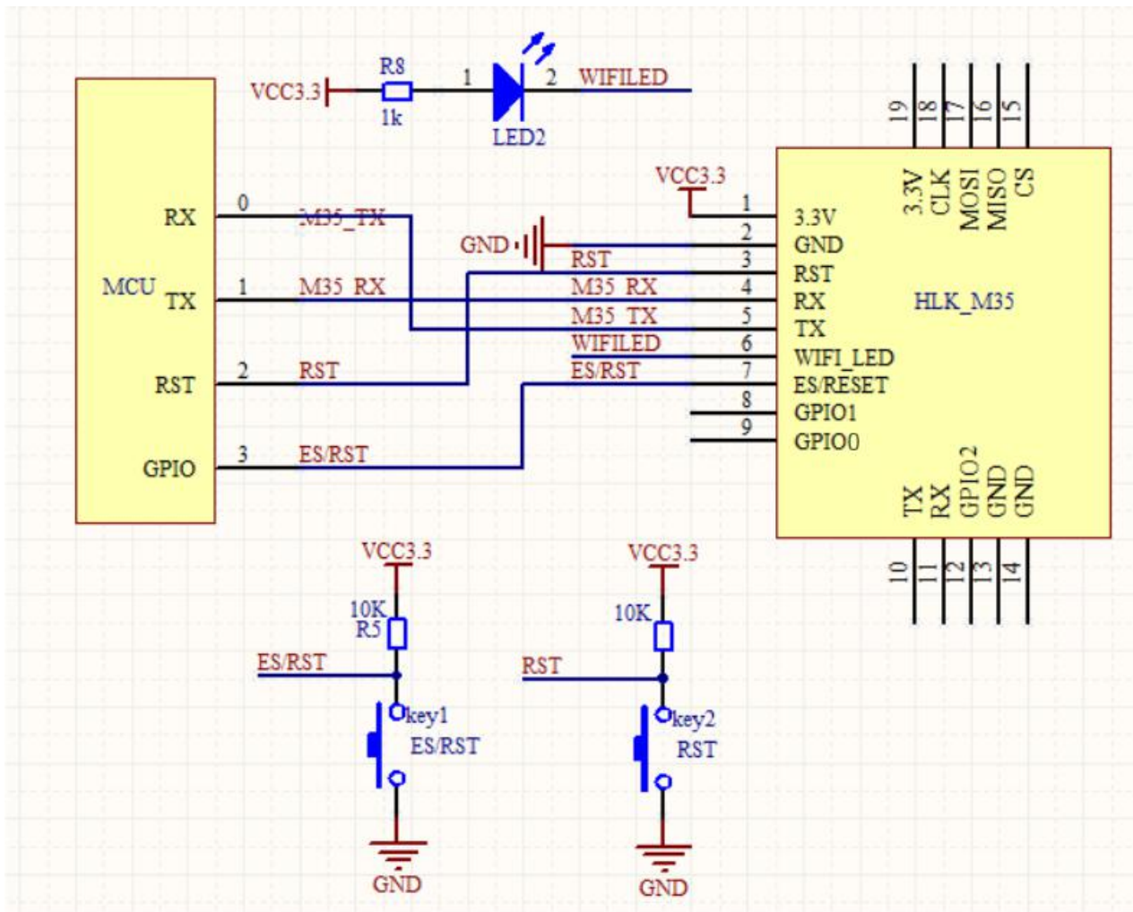
Figure 7. HLK-M35 硬件连接典型应用
