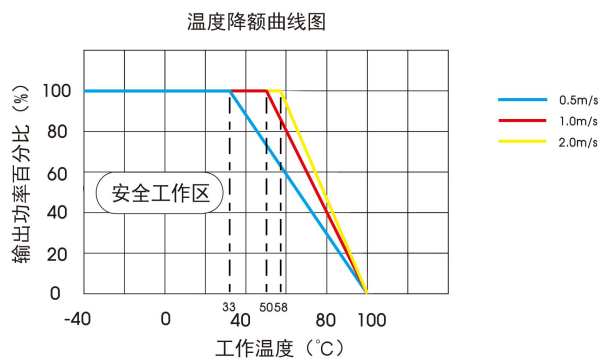
VCB4828EBO-100WR3 (Vin=48V)
