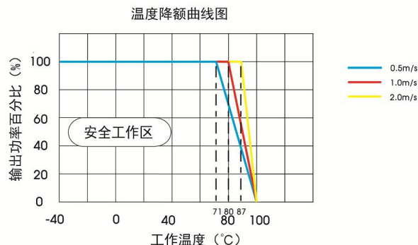
VCB4812EBO-100WR3 (Vin=48V)
